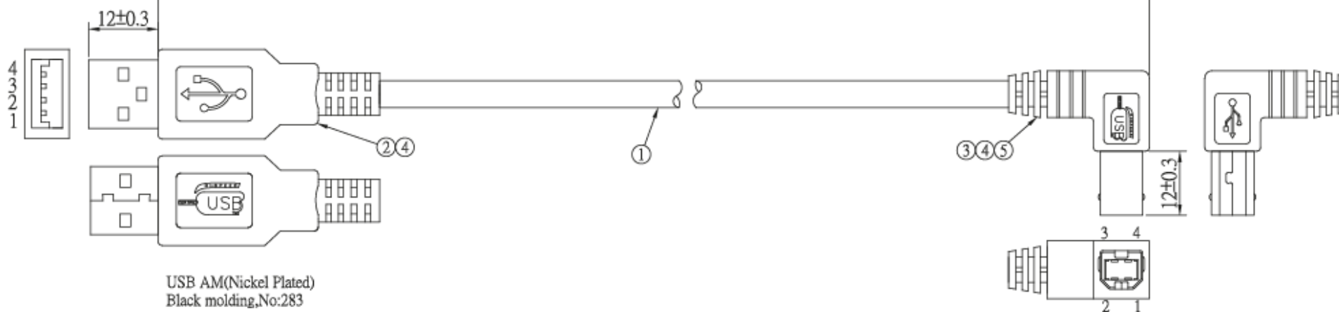
USB BM(Nickel Plated) Black molding,No:063
