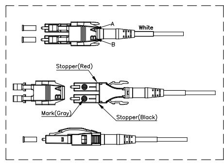
Polarity Twist LC Connector(SCALE 1/2)
