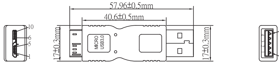
MICRO USB BM(NICKEL PLATED)
