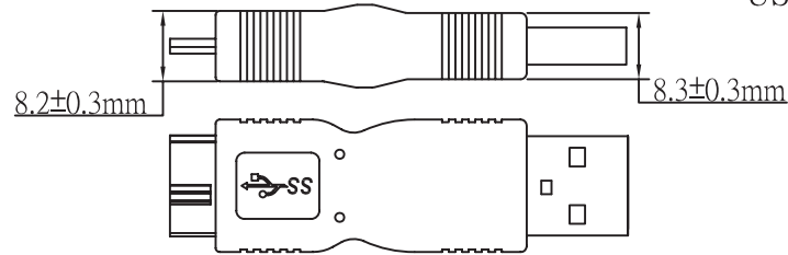
MICRO USB BM TO USB AM ADAPTER BLUE MOLDING
