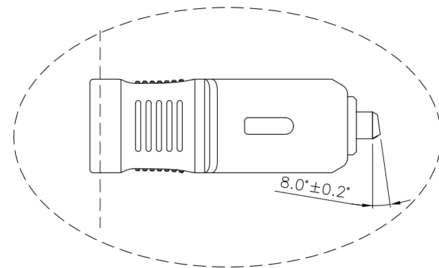
SC/APC Angles(SCALE 2/1)
