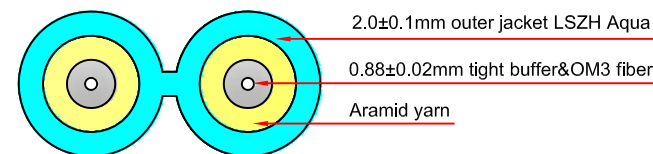
DETAIL D
