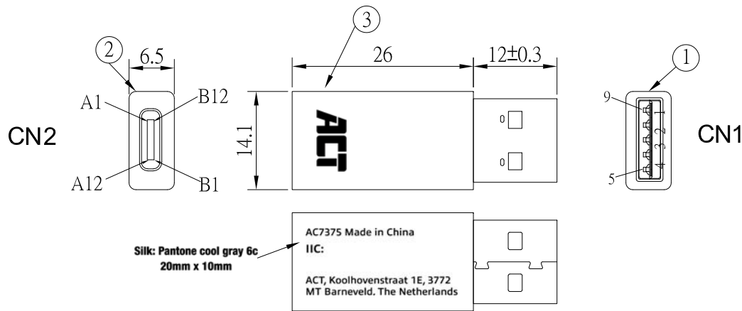
USB3.0 AM-Type CF Adapter Silver Metal Assembly Shell TOL:±0.5mm
